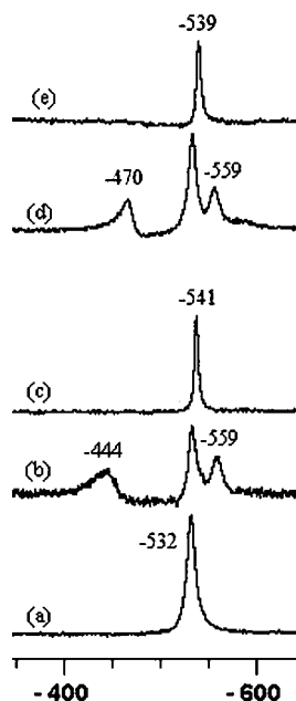
Figure 4. ^{51}\text{V} NMR spectra for \text{Cs}_2[\text{CH}_2\{\text{V}^{\text{VO}}\text{O}_2(\text{sal-nah})\}_2]\cdot 2\text{H}_2\text{O} ( 4 ): (a) in dmsO and after additions of aqueous acids: (b) 2.0 equiv. \text{HCl} and (d) 2.0 equiv. \text{HClO}_4 . Upon addition of MeOH to the solutions of spectra (b) and (d) so that the mixtures contain equal volumes of MeOH and dmsO, spectra (c) and (e), respectively, were recorded.
