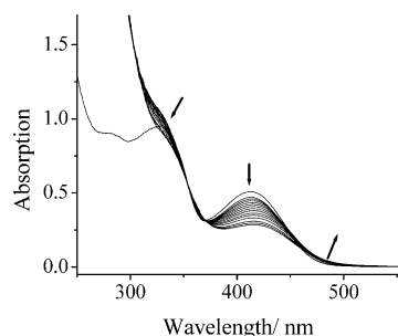
Figure 7. UV/Vis spectrum of 20 mL of an approximately 4.135 \times 10^{-5} M methanolic solution of \text{Cs}_2[\text{CH}_2\{\text{VVO}_2(\text{sal-inh})\}_2] \cdot 2\text{H}_2\text{O} ( 5 ) and spectral changes observed with time after addition of 30% aqueous \text{H}_2\text{O}_2 (30 drops, 18.04 mmol). Each spectrum was recorded at 25-min intervals.
