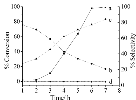
Figure 9. Conversion of methyl phenyl sulfide and variation in the selectivity of different reaction products as a function of time with 1 as catalyst: (a) conversion of methyl phenyl sulfide, (b) selectivity of methyl phenyl sulfoxide, (c) selectivity of methyl phenyl sulfone and (d) other unidentified product.
