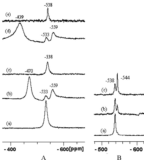
Figure 2. ^{51}\text{V} NMR spectra for \text{K}_2[\text{CH}_2\{\text{VVO}_2(\text{sal-nah})\}_2]\cdot 2\text{H}_2\text{O} ( 3 ). (A): (a) in dmsO (about 4 mM), (b) solution of (a) after addition of 3.0 equiv. of an aqueous solution of \text{HClO}_4 (15.8 M), the pH being about 3.1; (c) solution of (b) after addition of MeOH, the solution now containing equal volumes of dmsO and MeOH; (d) solution of (a) after addition of 3.0 equiv. of an aqueous solution of \text{HCl} (11.6 M), the pH being about 3.3; (e) solution of (d) after addition of MeOH, the solution now containing equal volumes of dmsO and of MeOH. (B): ^{51}\text{V} NMR spectra of 3 (a) in MeOH, about 4 mM; (b) after addition of 2.0 equiv. of an aqueous solution of \text{HCl} (11.6 M); (c) solution of spectrum (b) after standing for about 15 h.
