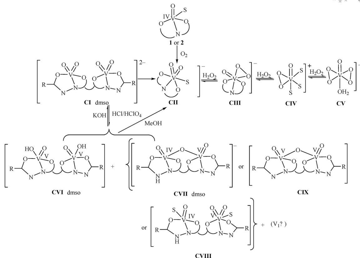
Scheme 3. Summary of speciation of vanadium species in solution.
