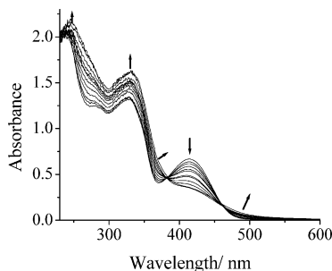
Figure 8. Spectral changes obtained during titration of 20 mL of a 6.535 \times 10^{-5} M methanolic solution of \text{Cs}_2[\text{CH}_2\{\text{VVO}_2(\text{sal-inh})\}_2] \cdot 2\text{H}_2\text{O} ( 5 ) with HCl gas saturated in methanol; the spectra were recorded after the successive additions of one-drop portions.
