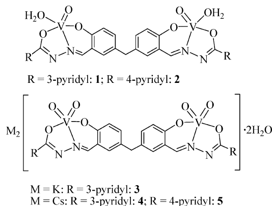
Scheme 2. Schematic structure of the V IV O and V V O 2 complexes prepared.
