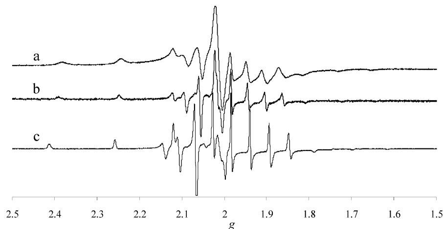
Figure 6. First-derivative EPR spectra (at 77 K) of a solution of [\text{CH}_2\{\text{VO}(\text{sal-nah})(\text{H}_2\text{O})\}_2] ( 1 ): (a) in dmso (about 4 mM); (b) after addition of an equal volume of MeOH; and (c) after addition of 0.5 equiv. of an aqueous 30% \text{H}_2\text{O}_2 solution.
