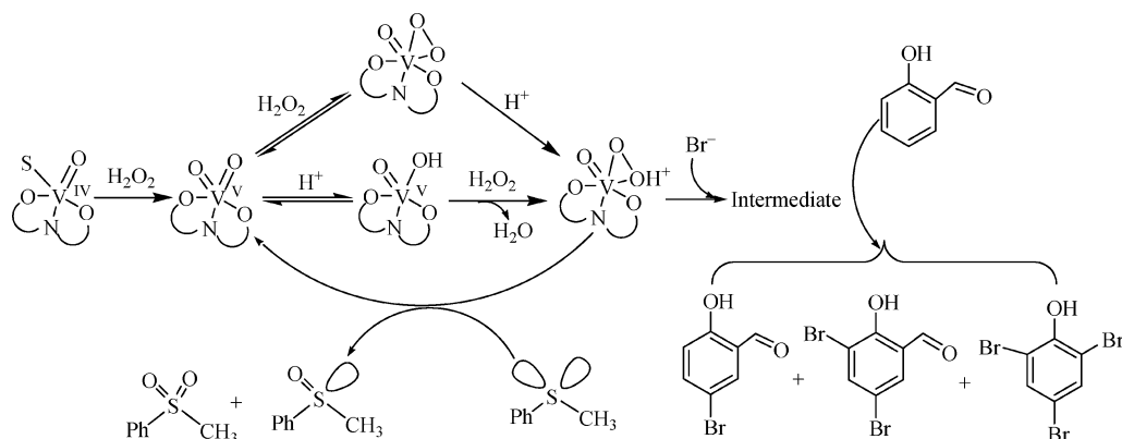
Scheme 5. Outline of the catalytic processes.
