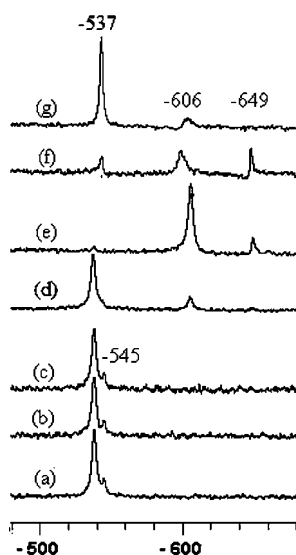
Figure 3. ^{51}\text{V} NMR spectra for \text{Cs}_2[\text{CH}_2\{\text{V}^{\text{VO}}\text{O}_2(\text{sal-nah})\}_2]\cdot 2\text{H}_2\text{O} ( 4 ): (a) in MeOH (about 4 mm of 4 ) and upon stepwise addition of aqueous 30% solution \text{H}_2\text{O}_2 ; (b) 1.0 equiv. \text{H}_2\text{O}_2 ; (c) 4.0 equiv. \text{H}_2\text{O}_2 ; (d) 6.0 equiv. \text{H}_2\text{O}_2 ; (e) 8.0 equiv. \text{H}_2\text{O}_2 ; (f) solution of (e) after 24 h leaving the tube open; (g) solution of (e) after 36 h of leaving the tube open.
