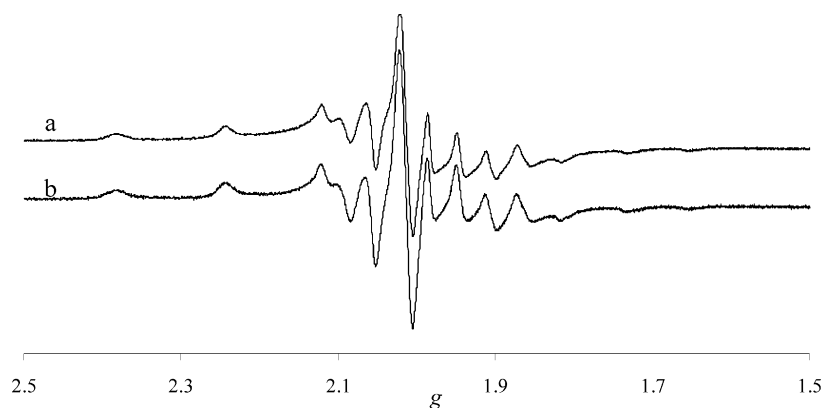
Figure 5. EPR spectra of frozen solution (4 mm) samples of [\text{CH}_2\{\text{V}^{\text{IV}}\text{O}(\text{sal-nah})(\text{H}_2\text{O})\}_2] ( 1 ) (a) and [\text{CH}_2\{\text{V}^{\text{IV}}\text{O}(\text{sal-inh})(\text{H}_2\text{O})\}_2] ( 2 ) (b) in dmso.
