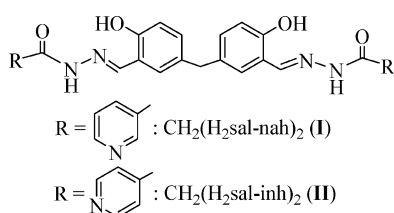
Scheme 1. Structures of ligands designated by I and II used in this work.
