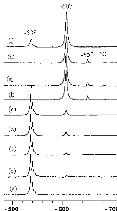
Figure 1. 51 V NMR spectra for solutions (about 4 mM) of K 2 [CH 2 {V VO O 2 (sal-nah)} 2 ]·2H 2 O ( 3 ): (a) in MeOH and (b–h) after stepwise additions of an aqueous solution of 30% H 2 O 2 ; (b) 0.5 equiv. H 2 O 2 added; (c) 2 equiv. H 2 O 2 (total) added; (d) 4.0 equiv. H 2 O 2 (total) added; (e) 6.0 equiv. H 2 O 2 (total) added; (f) 8.0 equiv. H 2 O 2 (total) added; (g) 10 equiv. H 2 O 2 (total) added; (h) solution of (g) after 2 h leaving tube open; (i) solution of (h) after 36 h leaving tube open.
